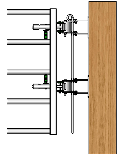
Broche anti-passage / Bare pin BA9931 (trou à re-percer / hole to re-drill Ø15)
