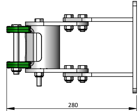
Montage / Mounting maxi
