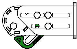
Montage / Mounting 45°
